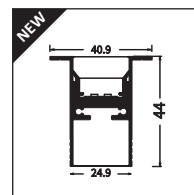
AL5 (1Mtr) CONCEALED Aluminium Profile Base Suitable for PRO-258
