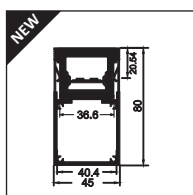
AL7 (1Mtr) Aluminium Profile Base Suitable for PRO-259
