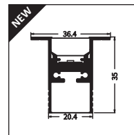
AL2 (1Mtr) CONCEALED Aluminium Profile Base Suitable for PRO-257
