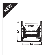
AL8 (1Mtr) Aluminium Profile Base Suitable for PRO-259
