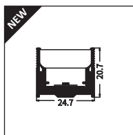
AL4 (1Mtr) Aluminium Profile Base Suitable for PRO-258
