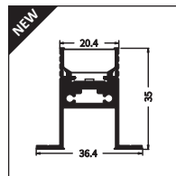
AL2 (1Mtr) - INGROUND Aluminium Profile Base Suitable for PRO-257
