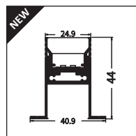
AL5 (1Mtr) - INGROUND Aluminium Profile Base Suitable for PRO-258
