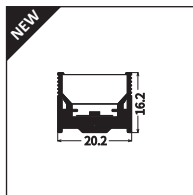
AL1 (1Mtr) Aluminium Profile Base Suitable for PRO-257
